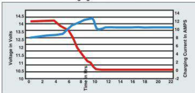
Charging Characteristics
