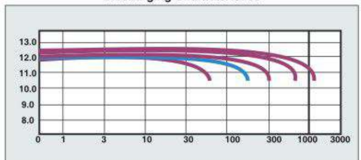
Discharging Characteristics
