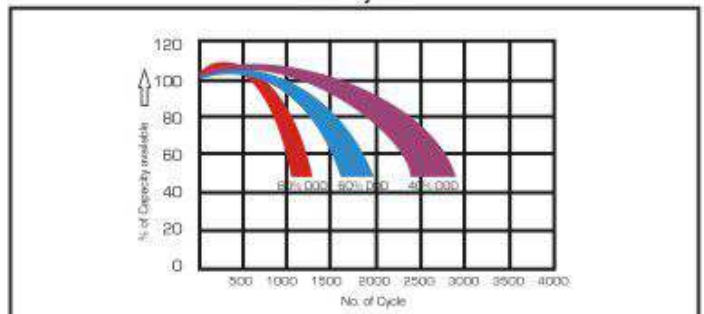
Life Cycle
