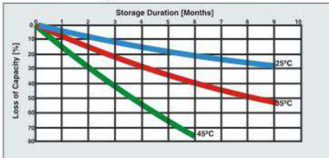
Self Discharge Characteristics - Tubular Batteries
